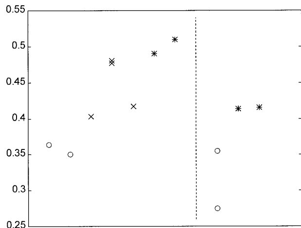
FIG. 6. Ratio of UVRRS peaks at 1330/1480 \text{cm}^{-1} . Symbols: same as those in Fig. 4.
